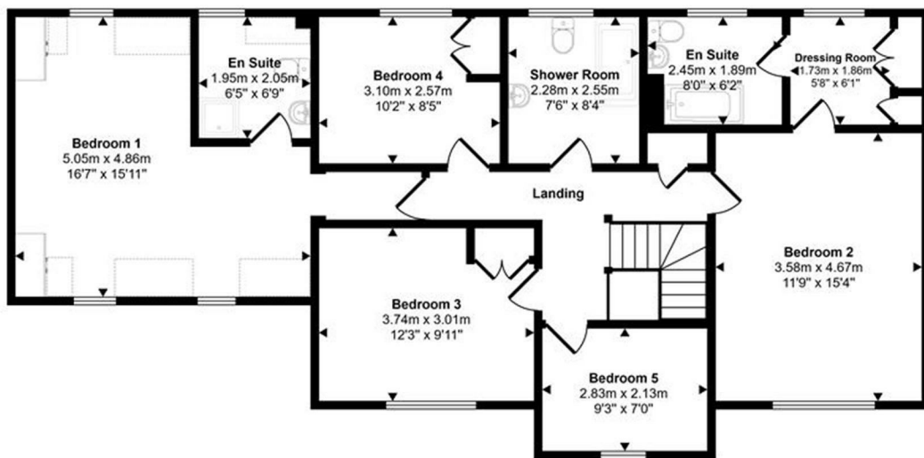
First Floor Approx 98 sq m / 1056 sq ft
